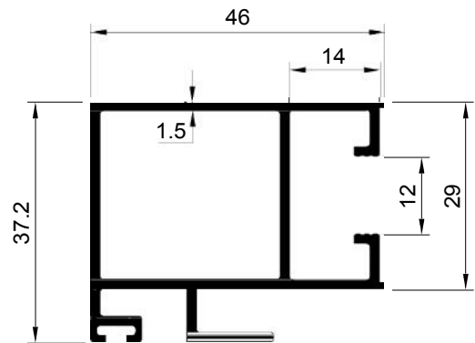
SECTION NO. - 80S-2601 EST. WEIGHT - 0.803 KG./M.
