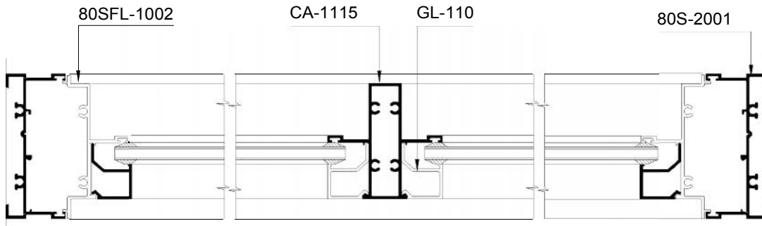
SECTION :- F - F
