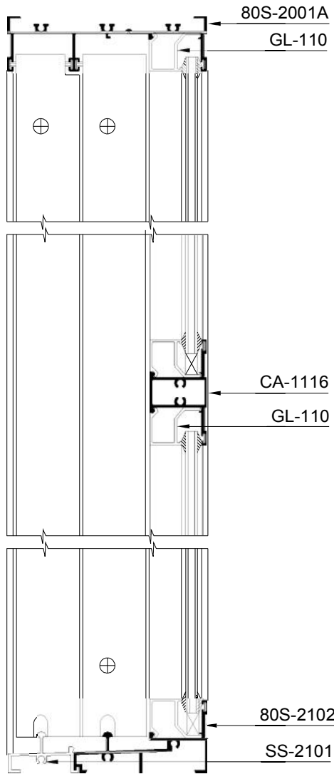
SECTION: - A-A
