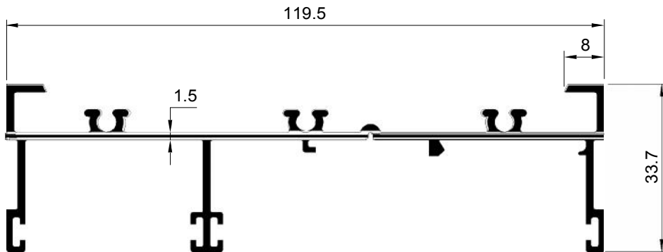
SECTION NO. - 80S-2001A EST. WEIGHT - 1.167 KG./M.
