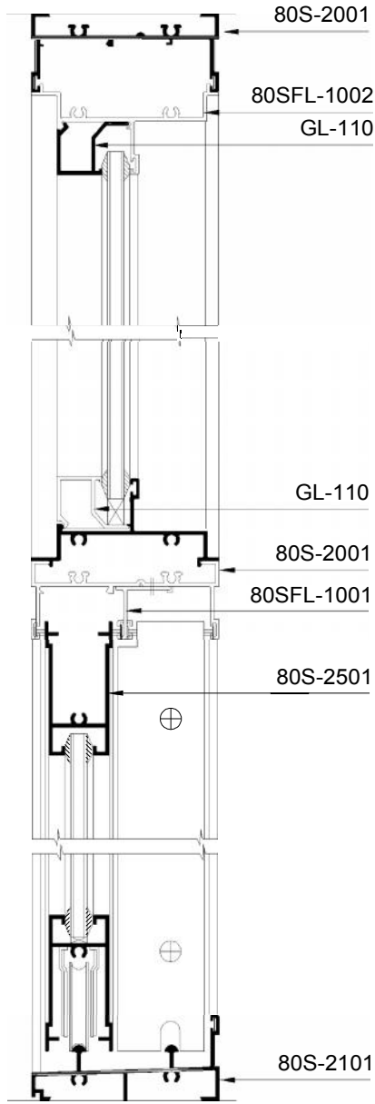
SECTION:- B-B
