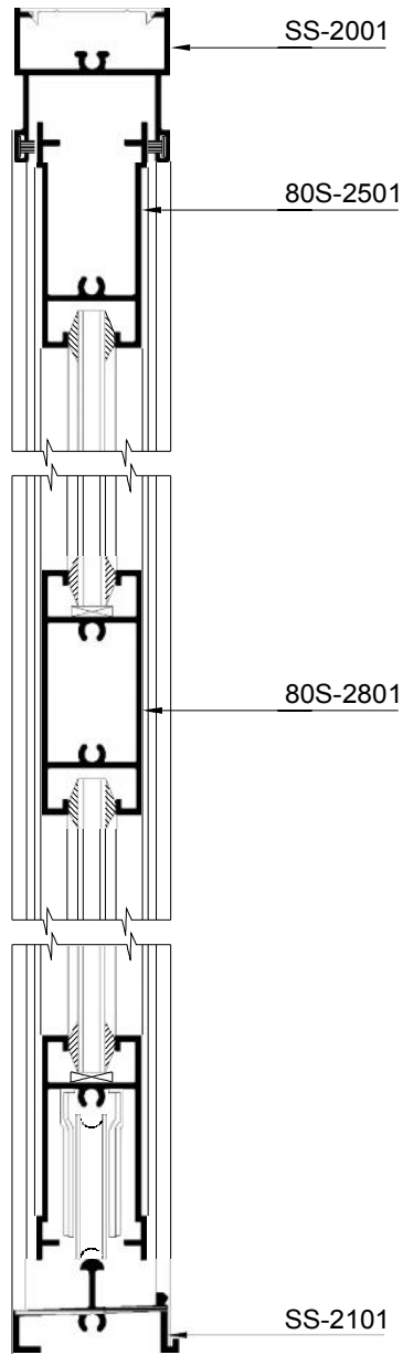
SECTION:-A-A
