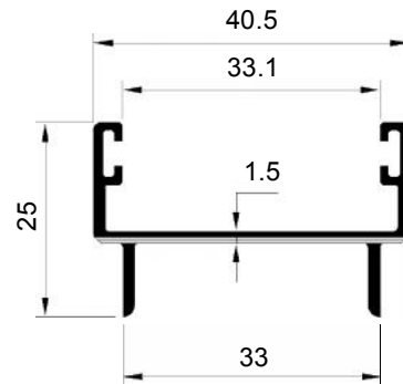
SECTION NO. - 80S-2901 EST. WEIGHT - 0.379 KG./M.
