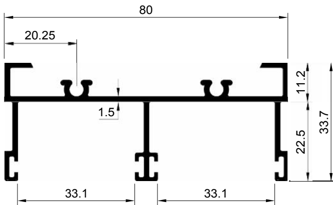
SECTION NO. - 80S-2002 EST. WEIGHT - 0.911 KG./M.
