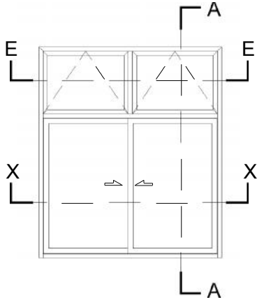
SLIDING WITH TOP HUNG
