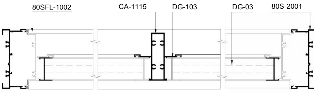
SECTION :- G - G
