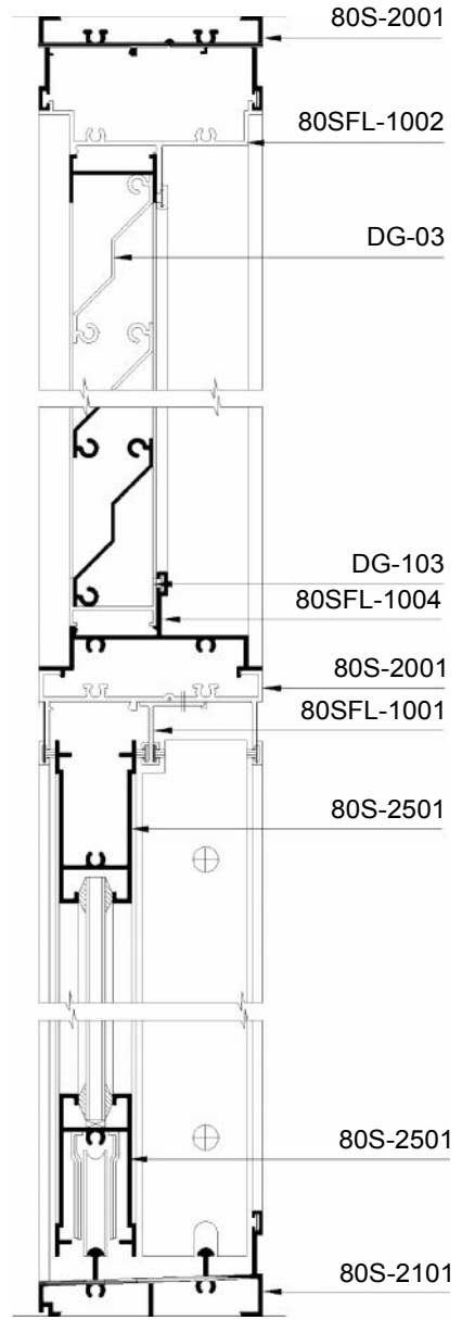
SECTION:- C-C
