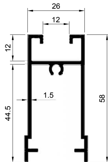
SECTION NO. - 80S-2501 EST. WEIGHT - 0.717 KG./M.
