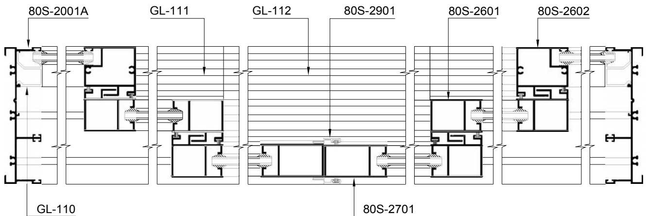
SECTION: - B-B
