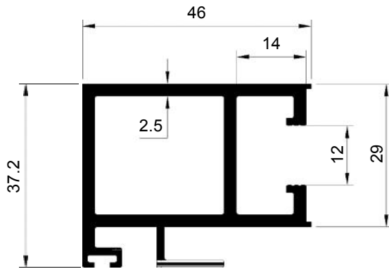
SECTION NO. - 80S-2601 H EST. WEIGHT - 1.194 KG./M.
